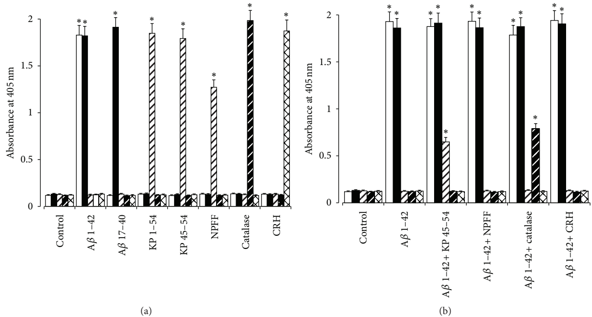
FIGURE 1: Binding of anti-A \beta , anti-KP, anti-catalase and anti-CRH antibodies to A \beta , KP, NPFf, catalase and CRH. In (a) plates were coated with A \beta 1-42, A \beta 17-40, KP 1-54, KP 45-54, NPFf, catalase, and CRH. Binding of BAM-10 mouse anti-A \beta antibody (open columns), rabbit anti-A \beta 21-32 antiserum (closed columns), rabbit anti-KP 45-54 antiserum (open hatched columns), CAT-505 mouse anti-catalase antibody (closed hatched columns) and KCHMB001 mouse anti-CRH antibody (open cross-hatched columns) was detected using alkaline phosphatase conjugated secondary antibodies and p-nitrophenylphosphate substrate. In (b) plates coated with A \beta 1-42 fibrils were preincubated with KP 45-54, NPFf, catalase, or CRH before addition of BAM-10 mouse anti-A \beta antibody (open columns), rabbit anti-A \beta 21-32 antiserum (closed columns), rabbit anti-KP 45-54 antiserum (open hatched columns) and CAT-505 mouse anti-catalase antibody (closed hatched columns), KCHMB001 mouse anti-CRH antibody (open cross-hatched columns). Binding was detected using alkaline phosphatase conjugated secondary antibodies and p-nitrophenylphosphate substrate. Results are expressed as mean \pm SEM ( n = 8 ) absorbance change at 405 nm. (* = P < 0.05 versus control; one-way ANOVA).
