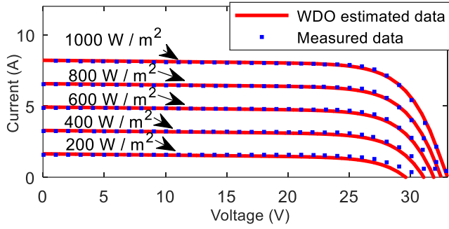
Fig. 7. Comparison of experimental data and WDO estimated data of Kyocera – KC200GT 215 module at different irradiance (double diode model).
