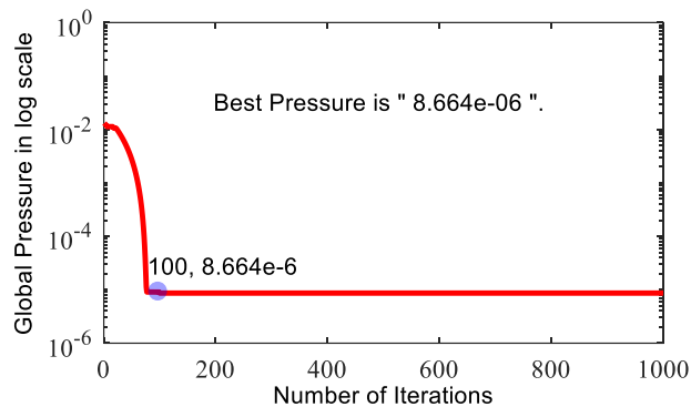
Fig. 9. Convergence curve of WDO algorithm for optimizing the parameters of single diode model
