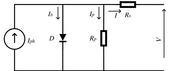
Fig. 1. Single – diode model of solar PV.
