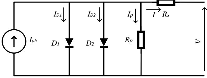
Fig. 2. Double – diode model of solar PV.
