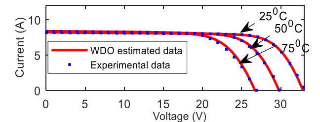
Fig. 6. Comparison of experimental data and WDO estimated data of Kyocera – KC200GT 215 module at different temperature (single diode model).
