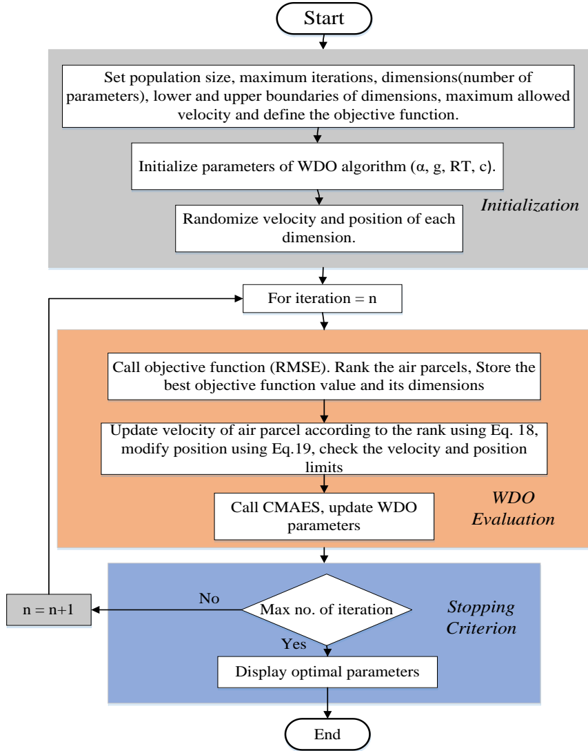
Fig. 3. Flowchart of Wind driven optimization
